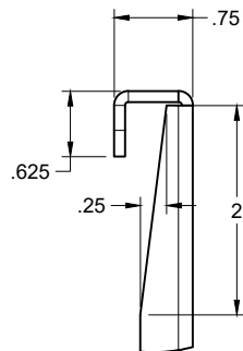
DETAIL A SCALE 1:2
