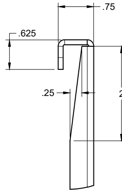
DETAIL A SCALE 1:2
